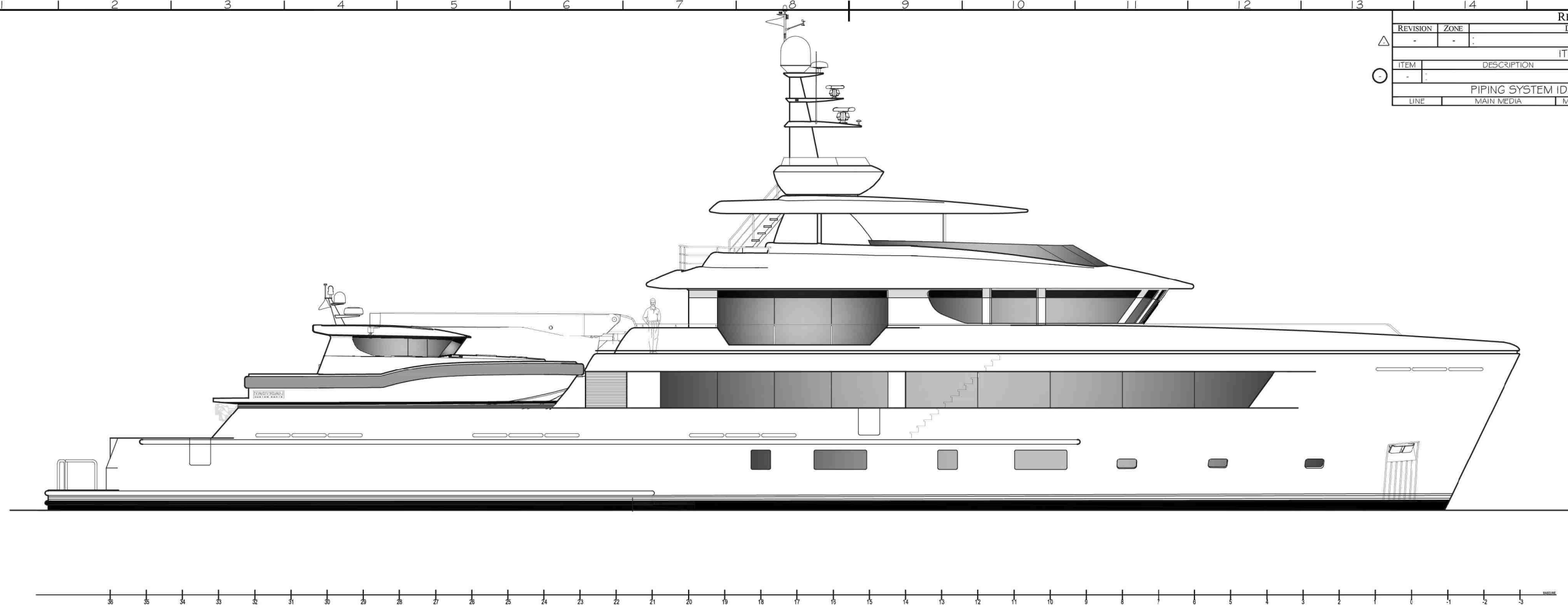
OUTBOARD PROFILE
