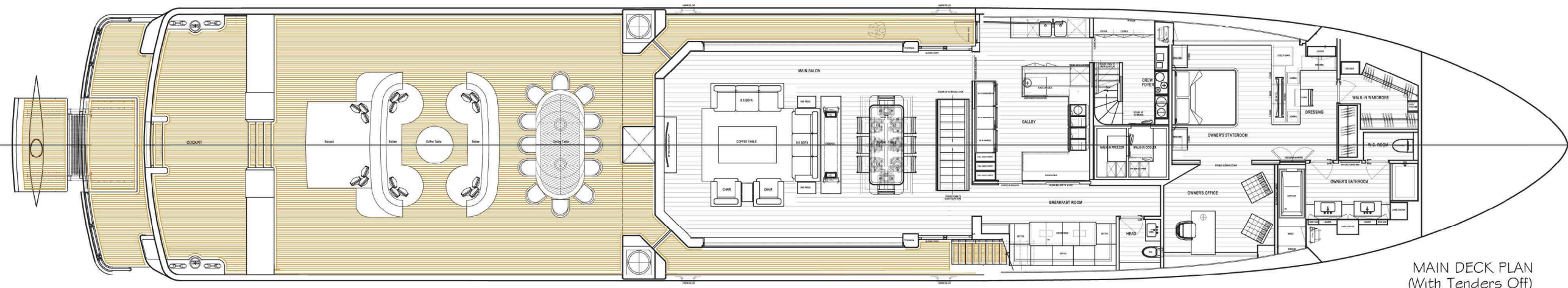
MAIN DECK PLAN (With Tenders On)
